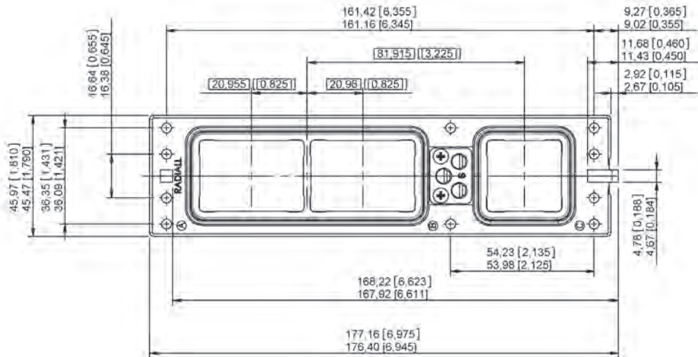
REAR VIEW
