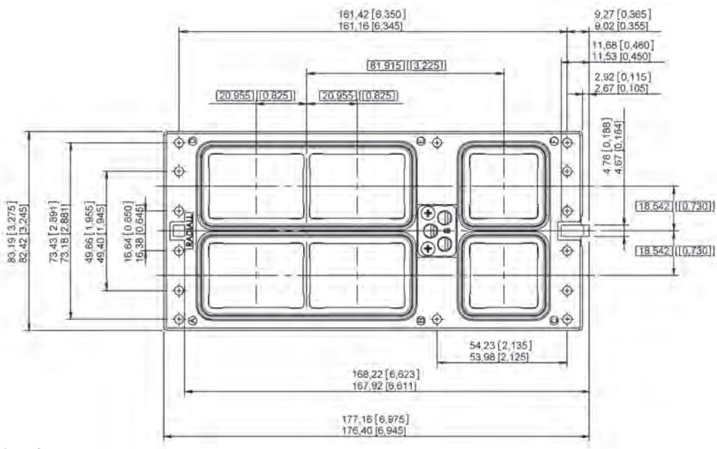
REAR VIEW
