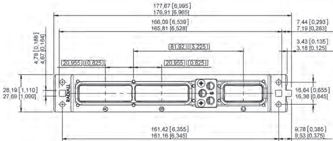
REAR VIEW
